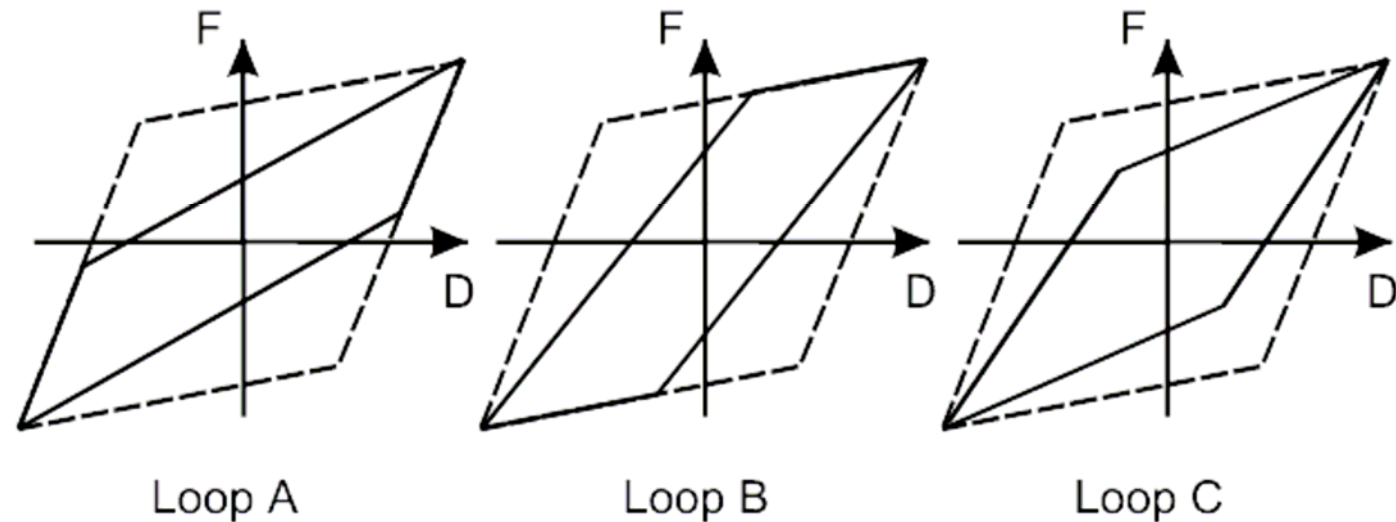
Figure 5.14 Loops with Same Energy Degradation
