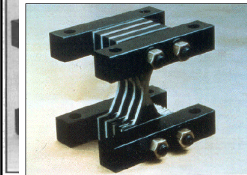
(a) X-shaped Plate Damper
