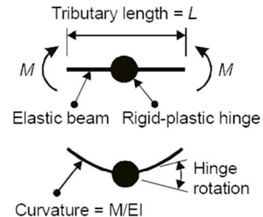
(b) Hinge Equivalent
