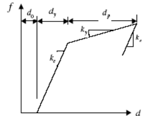
Tension-Gap-Yield element
