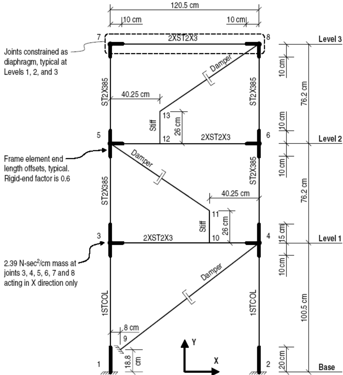
Damper Properties for Nonlinear Analyses
